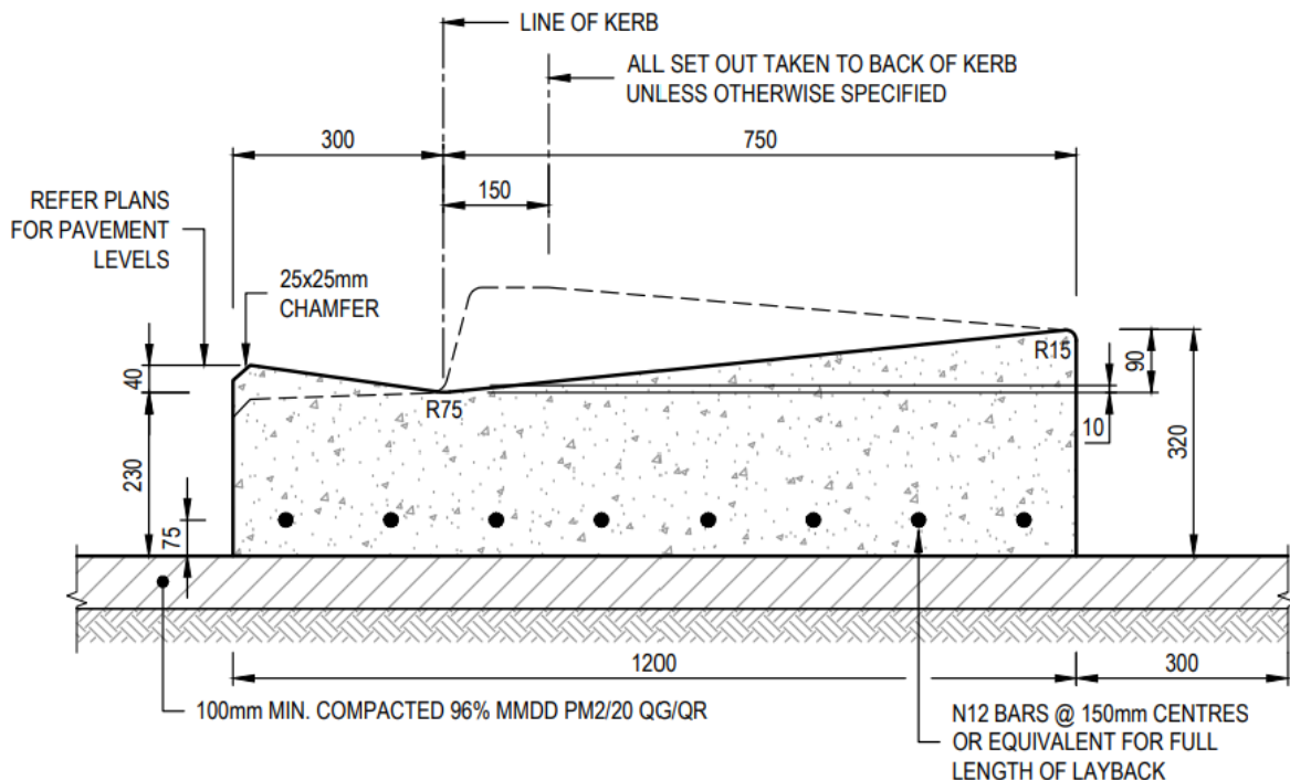
SECTIONAL VIEW OF INDUSTRIAL KERB LAYBACK
